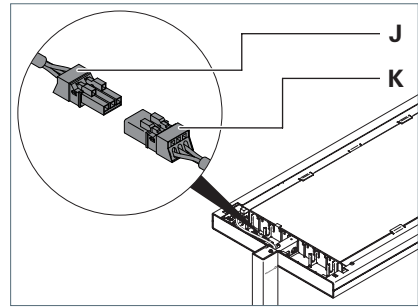
Fig. 5: Connecting the luminaire head, Part 2.
